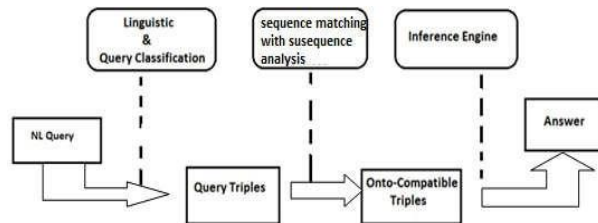
Fig. 1. Natural Language Query Processing
