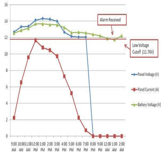
Figure 4: Manually Created Graph from Actual Measurements.
